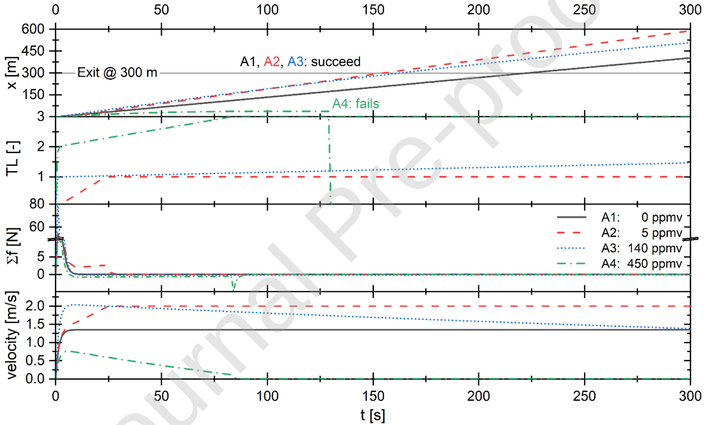
Figure 7 – Profiles of distance walked by the agent, x [m], toxic load, TL [-], total social force, f [N], and achieved speed, u [m.s -1 ] when exposed constantly to 0, 5, 140, & 450 ppmv for the A1, 2, 3, & 4 test cases. For clarity, note the break of force axis from 10 to 60 N.
